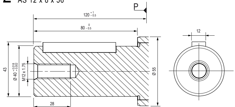
D2 Zylindrische Welle \varnothing 40 DIN 6885 AS 12 x 8 x 56
