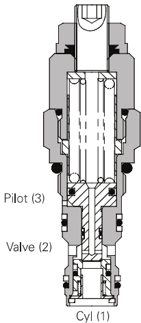
Sectional View
