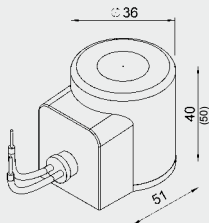
Connector type L Lead-wires, 457 mm
