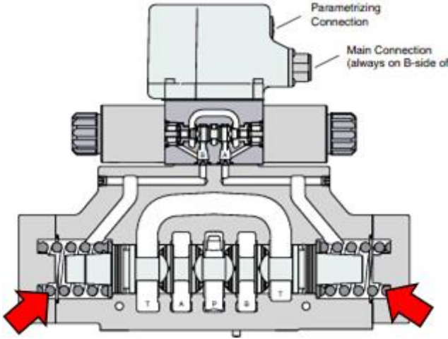
Feder D41FB-130/1240
