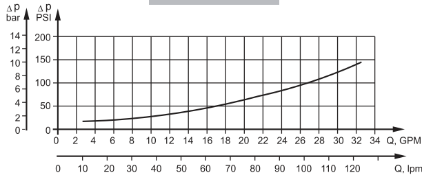
Pressure Losses
