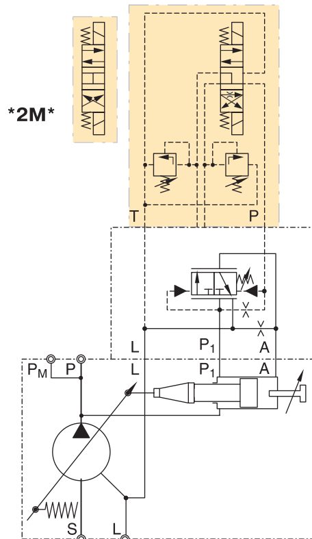
Schaltplan PVAC2M*/PVAC2E*
