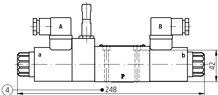
② Directional control valve with two solenoids and one switch
